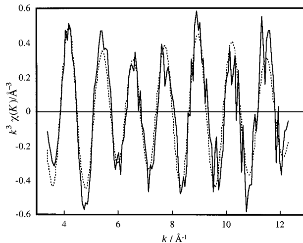
Fig. 4 Experimental EXAFS data (—) and structural model (---) of the cadmium K edge for the reaction medium [Et 3 S][I 2 ]–CdI 2 (10:1)
